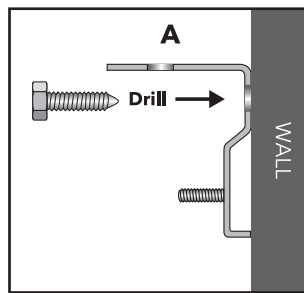
SIDE VIEW WALL MOUNT
