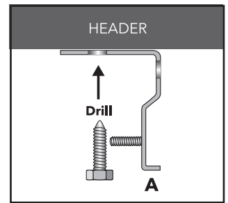
SIDE VIEW HEADER MOUNT
